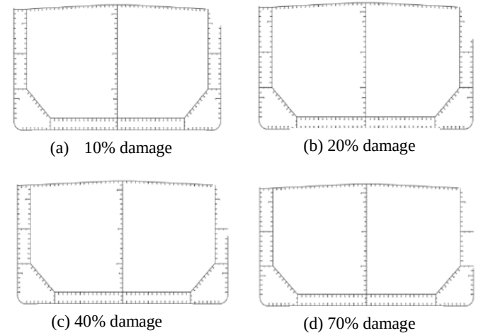
Fig. 3 Double hull oil tanker (Ship T2)
