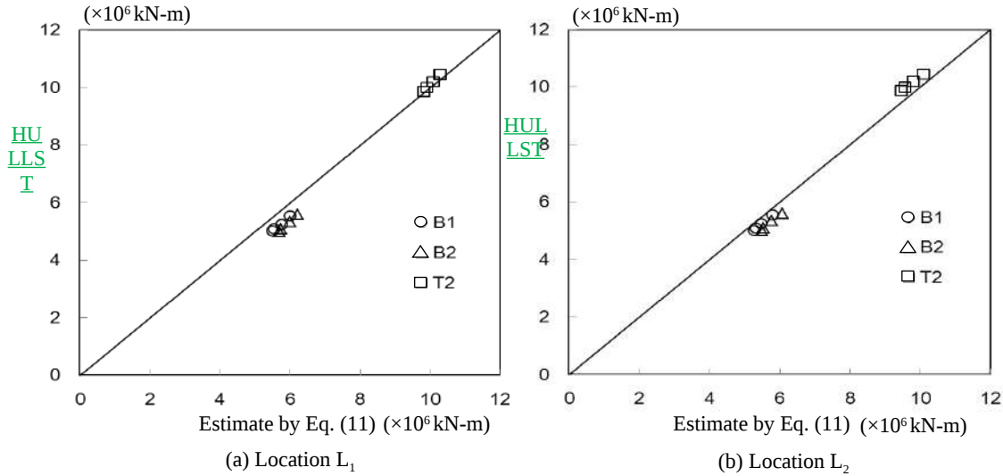
Fig. 11 Comparison of residual hull girder strength between the simplified method and the progressive collapse analysis
