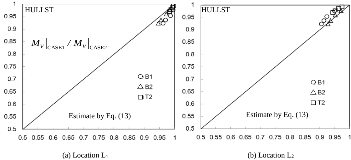
Fig. 12 Comparison of reduction ratio of residual hull girder due to rotation of neutral axis between the simplified method and the progressive collapse analysis (Case 1/Case 2)
