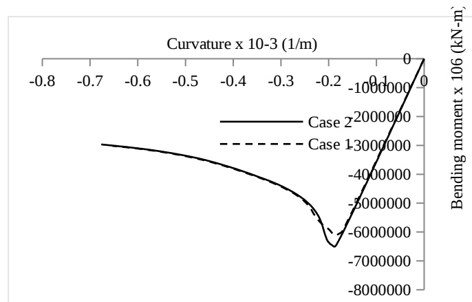
Fig. 8 Single-hull bulk carrier (Ship B2) with 70% damage
