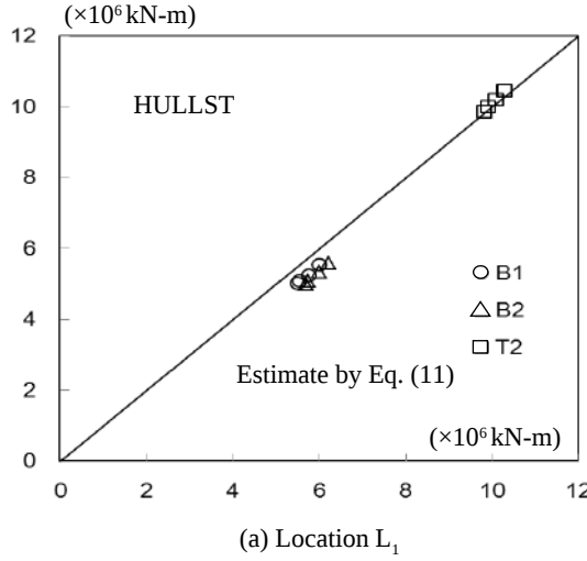
Fig. 11 Comparison of residual hull girder strength between the simplified method and the progressive collapse analysis
