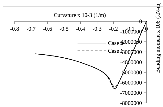
Fig. 7 Single-hull bulk carrier (Ship B2) with 20% damage
